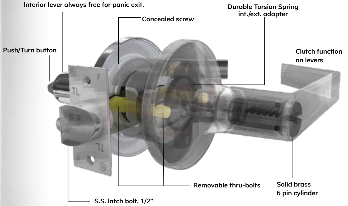
CT LEVER F Series Available in US26D
