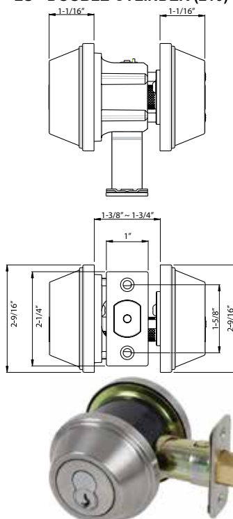
LU IC - SINGLE CYLINDER - IC CORE Shown in Satin Stainless Steel
