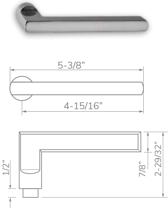
939 CHARLOTTE LEVER
