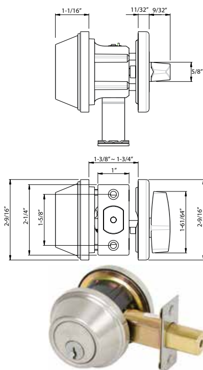
LU - SINGLE CYLINDER (200) Shown in Satin Stainless Steel
