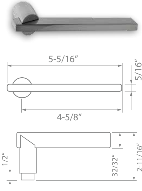
943 RALEIGH LEVER
