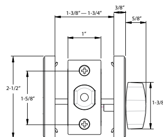
One-Sided Full Bore (206)
