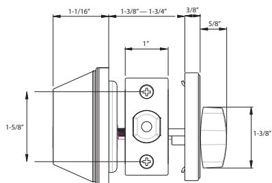
Single Cylinder (200)
